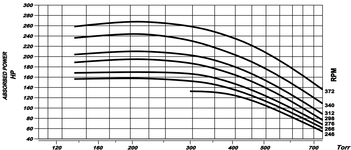
Service liquid at various Inlet pressure
