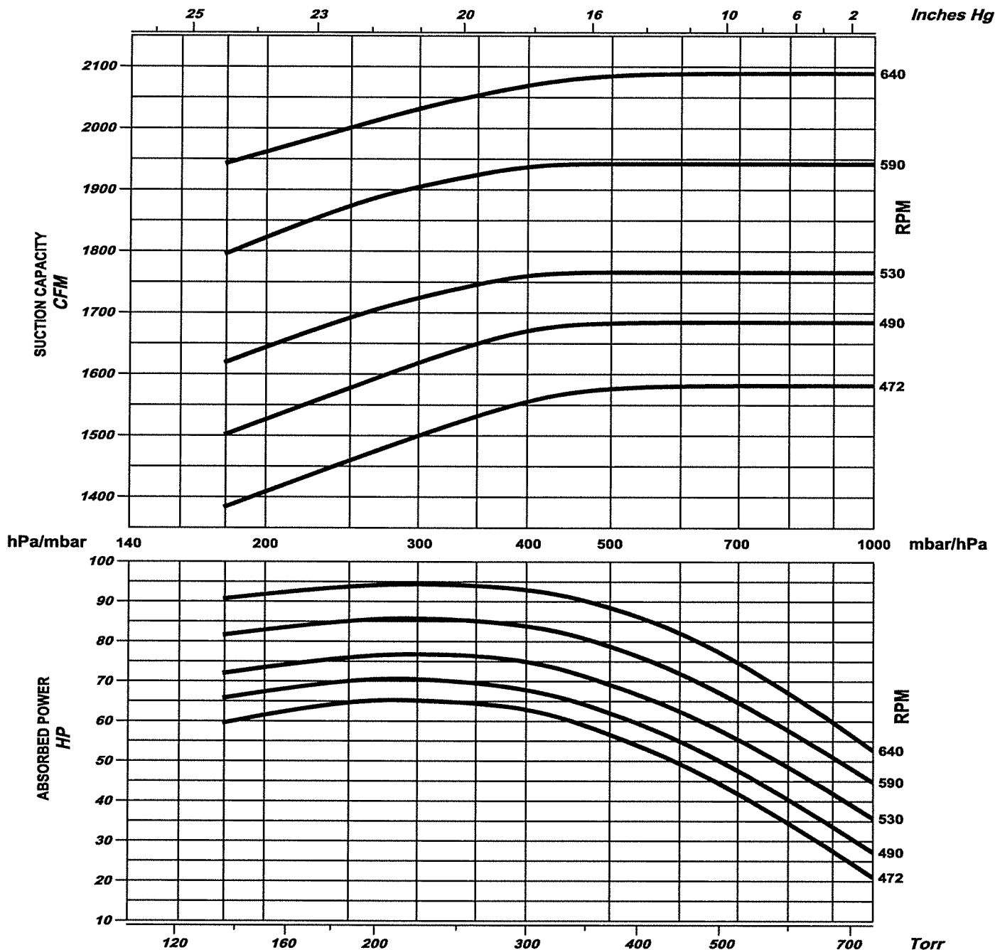
Service liquid at various Inlet pressure
