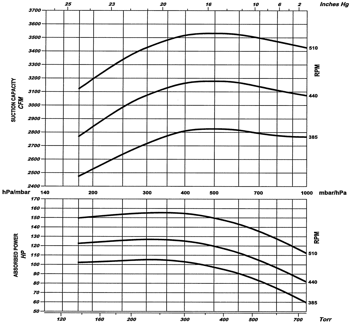
Service liquid at various Inlet pressure
