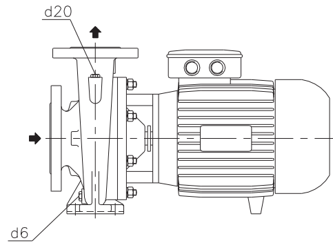
Pump series MCM Standard connections and hook-ups
