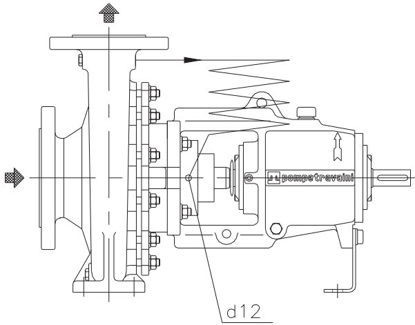
Fig. 12 - CONNECTIONS AND HOOK-UPS FOR FLUSHING
