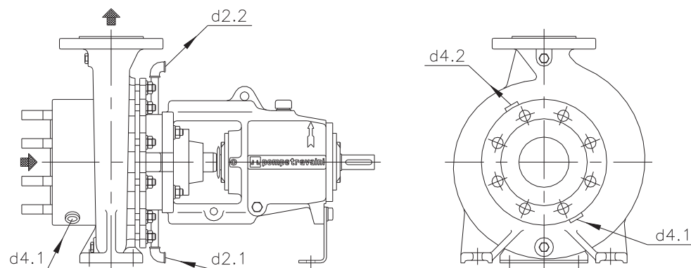
Pumps series MC... - TC... Connections for designs /T - /U2
