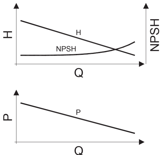
Typical performance curves for pumps series AT - TB...
