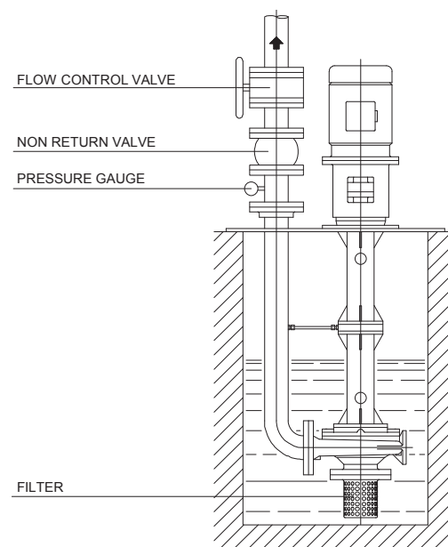
Pump series MC... - TC... - VERTICAL construction
