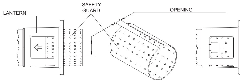
Fig. 15 - PREPARATION TO ASSEMBLY ON MONOBLOCK DESIGN
