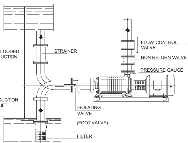
Pump series TBA - TBAK
